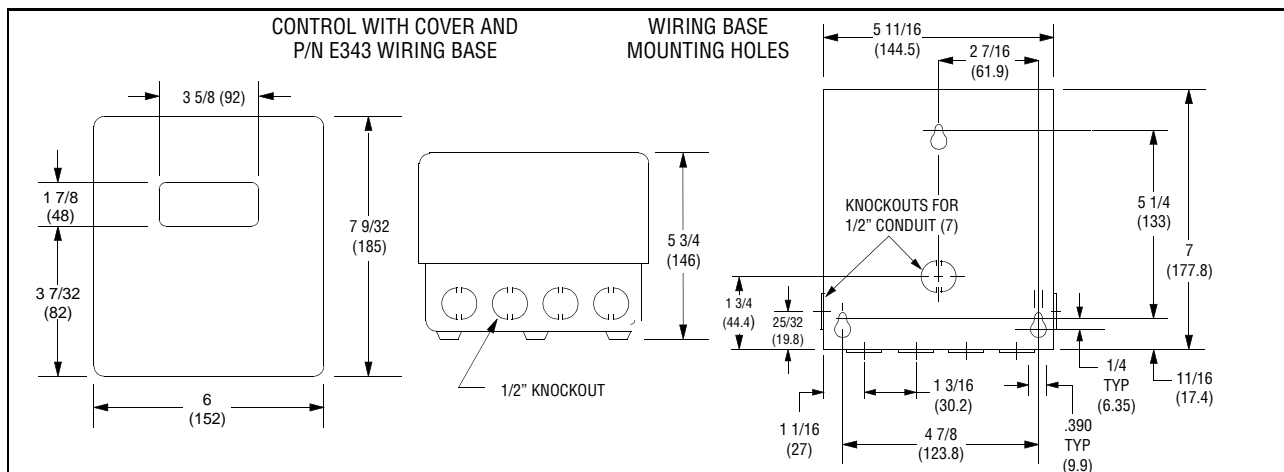
FIGURE 1. COMPONENT DIMENSIONS
